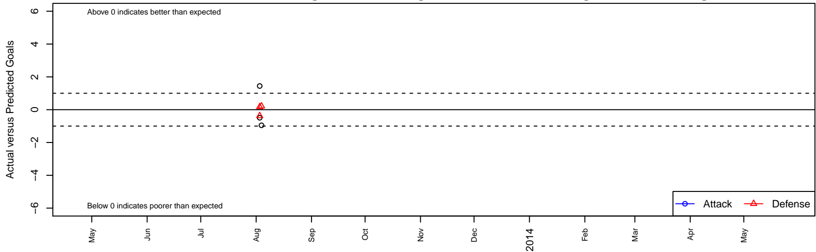
Albion FC Hurricanes 02 G01 Dots are actual minus expected GF (blue circles) and GA (red triangles). Blue line is smoothed change in attack strength. Red is smoothed change in defense strength.
